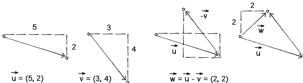
Figure 1.7: Vector Subtraction
