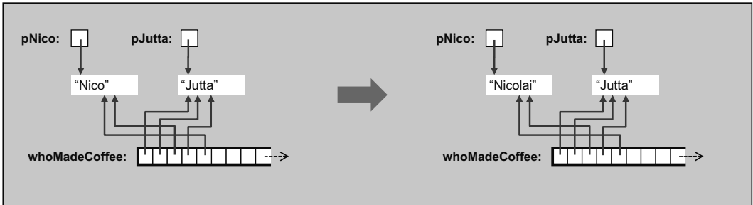
Figure 5.1. Using shared_ptr s
