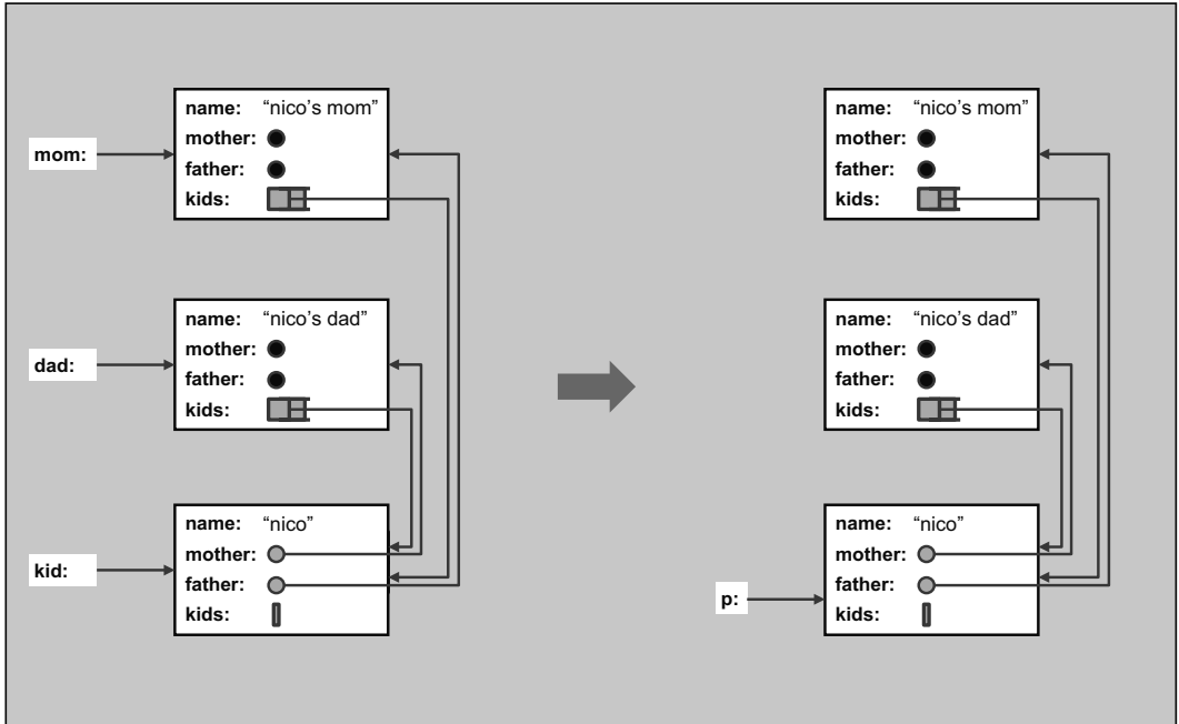
Figure 5.2. A Family Using shared_ptr Only
