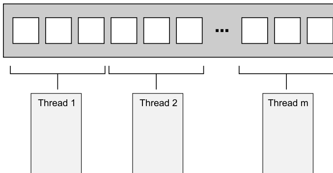
Figure 8.1 Distributing consecutive chunks of data between threads
