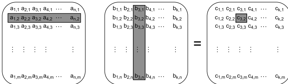
Figure 8.3 Matrix multiplication
