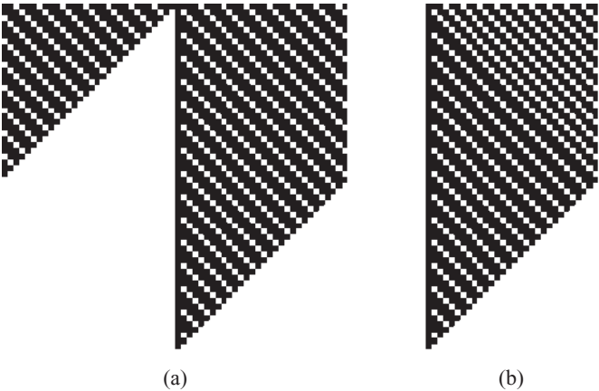
FIGURE 3.11 Rule 188: (a) ring; (b) line.
