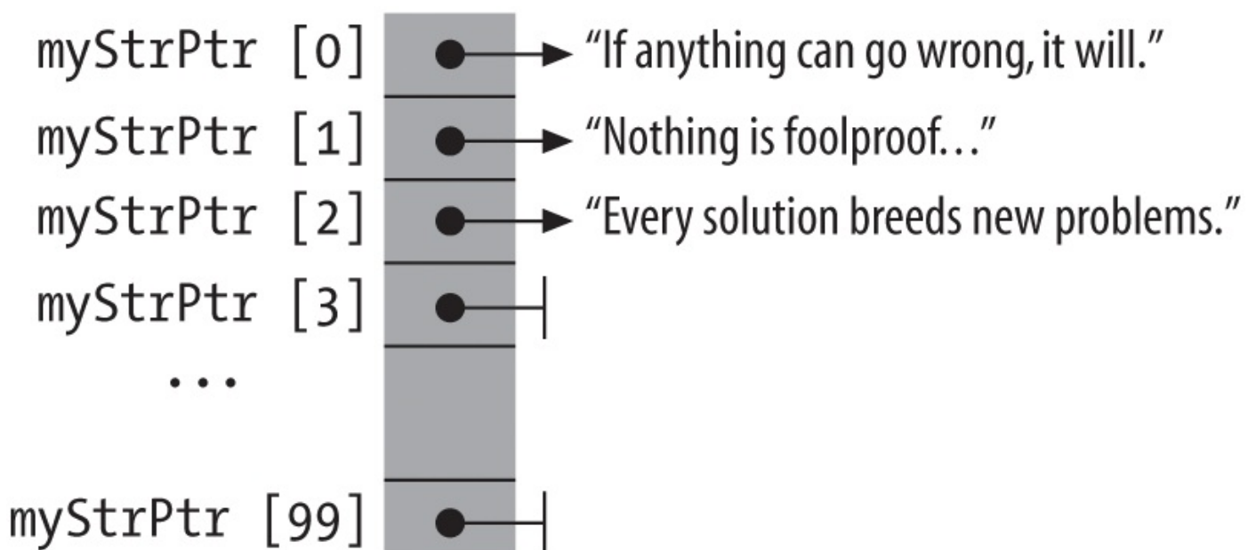
Figure 9-3. Pointer array
