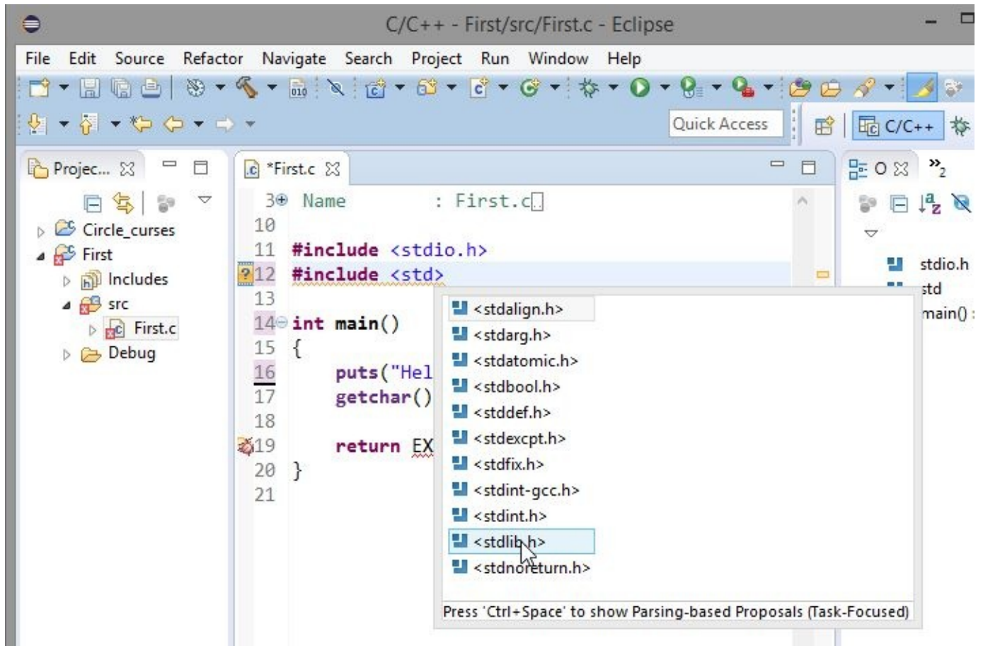
Figure 22-2. Code completion
