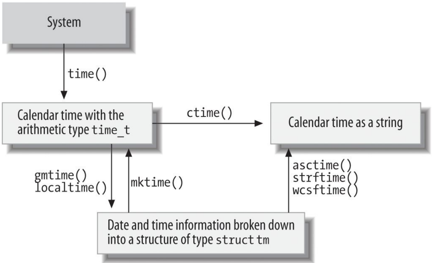
Figure 17-1. Date and time functions
