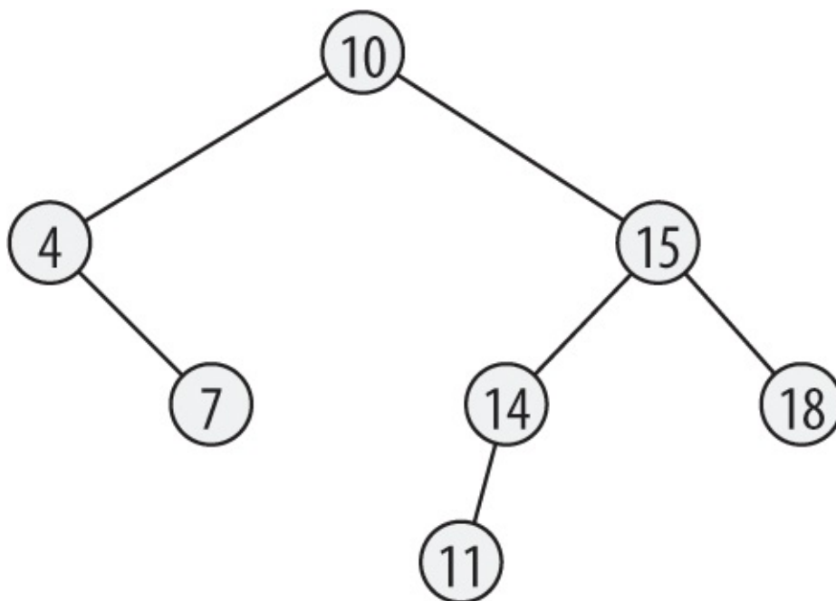
Figure 12-1. A binary tree
