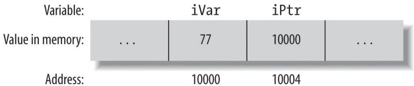
Figure 9-1. A pointer and another object in memory
