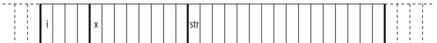
Figure 10-3. An object of the type struct Record in memory
