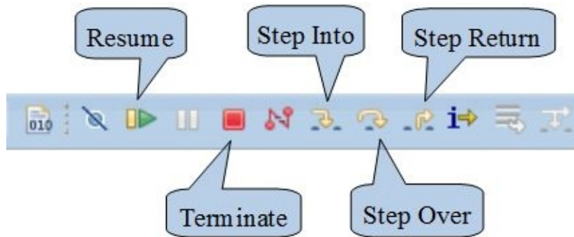
Figure 22-7. The Debug toolbar
