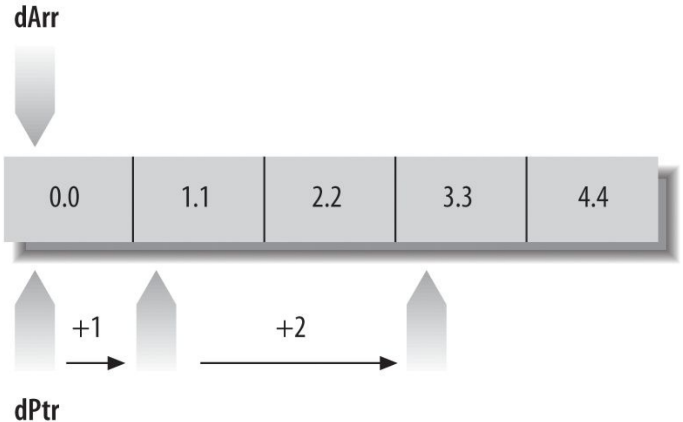
Figure 5-1. Using a pointer to move through the elements in an array
