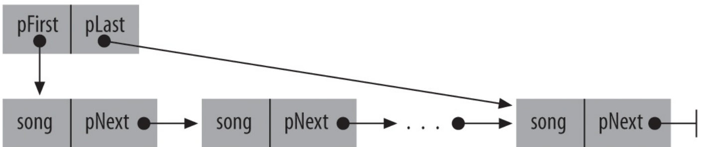
Figure 10-1. A singly linked list
