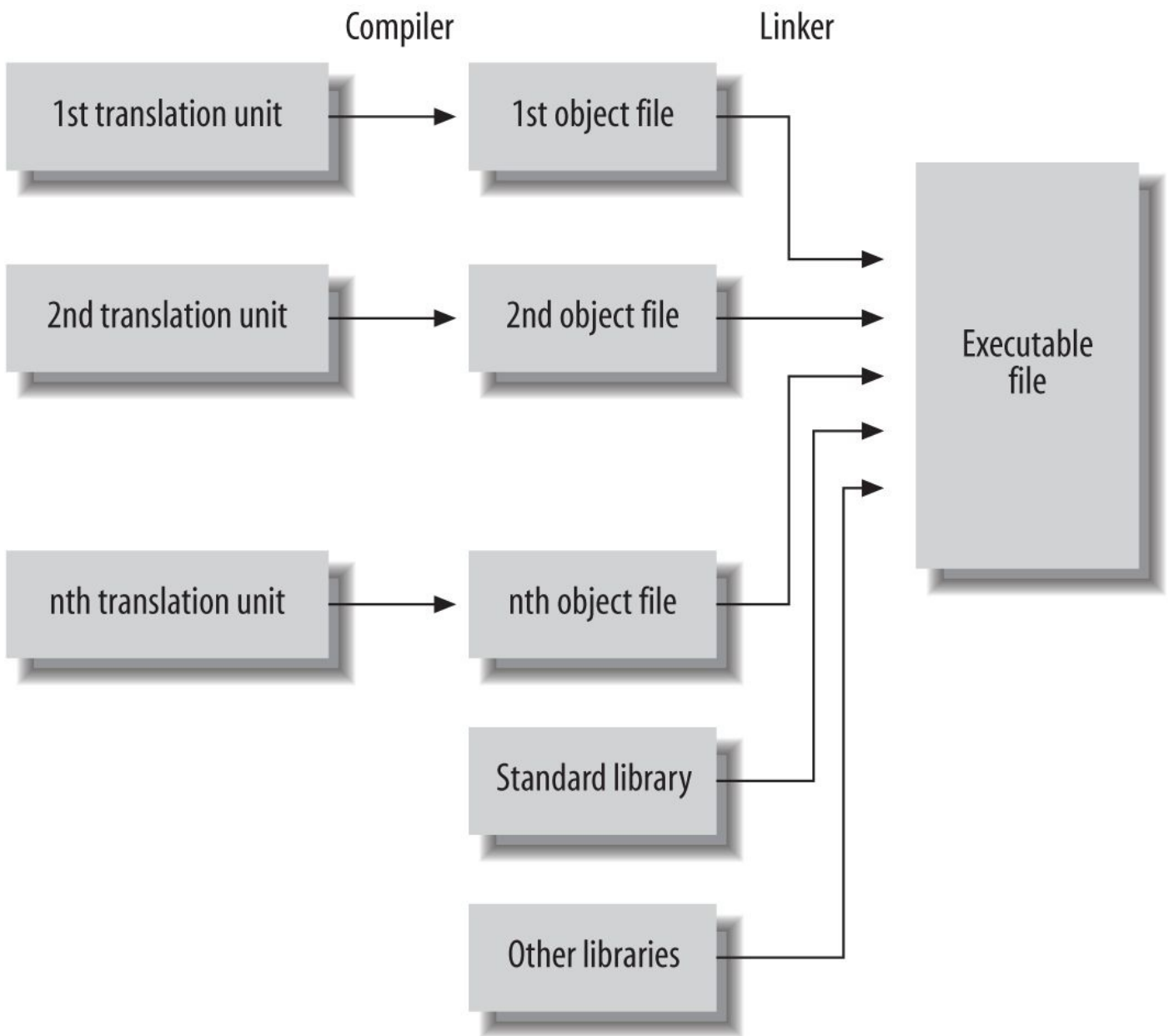
Figure 1-1. From source code to executable file
