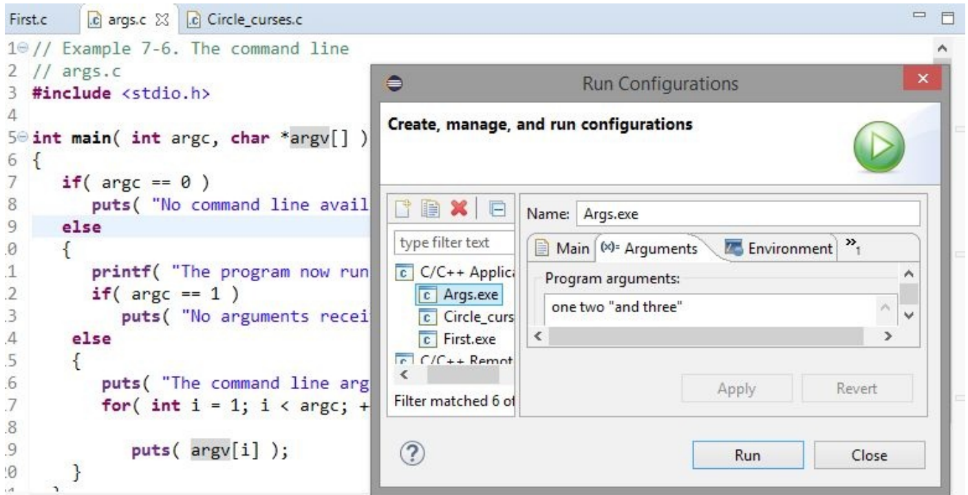
Figure 22-4. Run configuration
