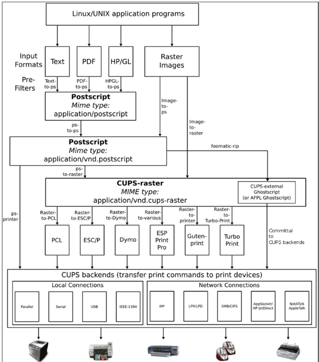
Figure 7-2. The Common Unix Printing System (CUPS) logical diagram. Glenn Davis (SVG), Ta bu shi da yu (PNG), and Kurt Pfeifle (ASCII) Creative Commons 9 Attribution-Share Alike 3.0 Unported 10 license.
