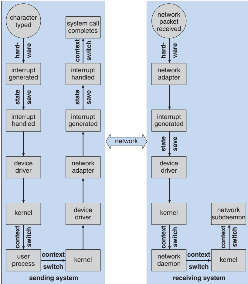
Figure 12.15 Intercomputer communications.
