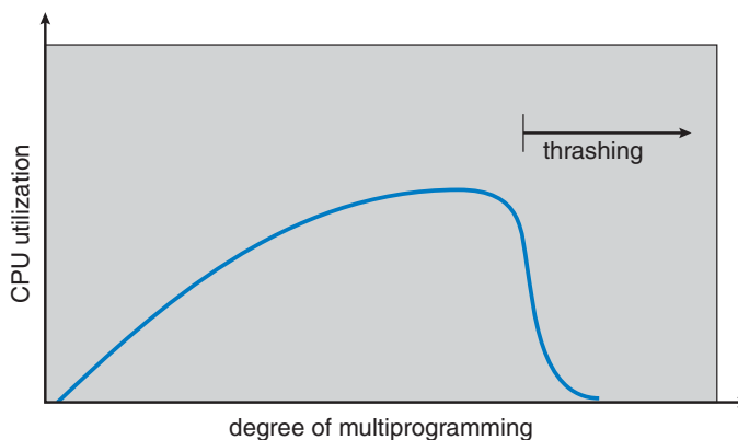
Figure 8.18 Thrashing.
