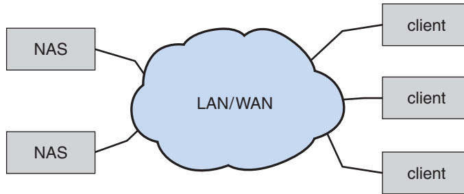
Figure 9.2 Network-attached storage.
