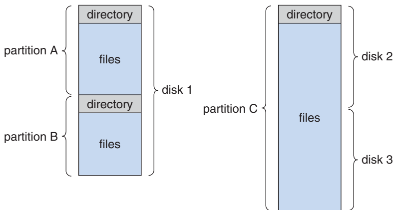
Figure 10.7 A typical file-system organization.
