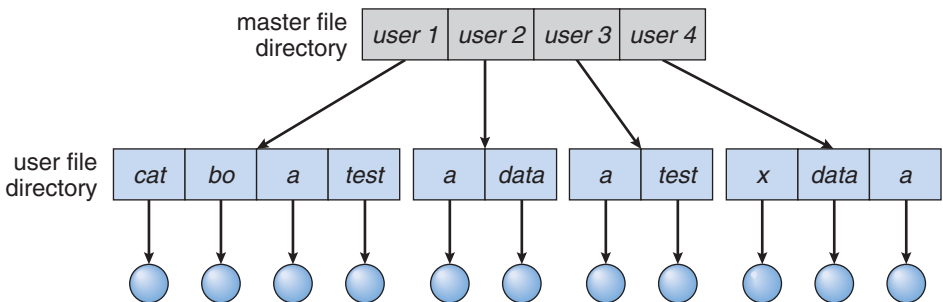
Figure 10.10 Two-level directory structure.
