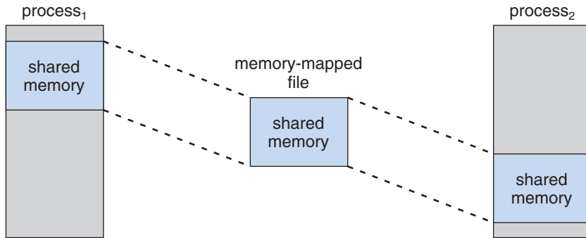
Figure 8.23 Shared memory using memory-mapped I/O.
