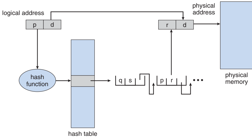
Figure 7.19 Hashed page table.
