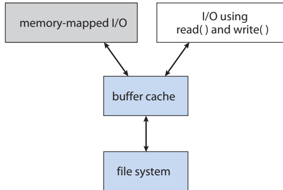
Figure 11.12 I/O using a unified buffer cache.
