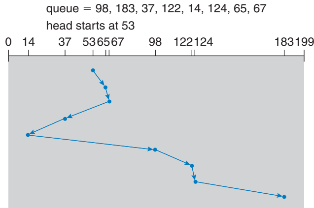
Figure 9.5 SSTF disk scheduling.
