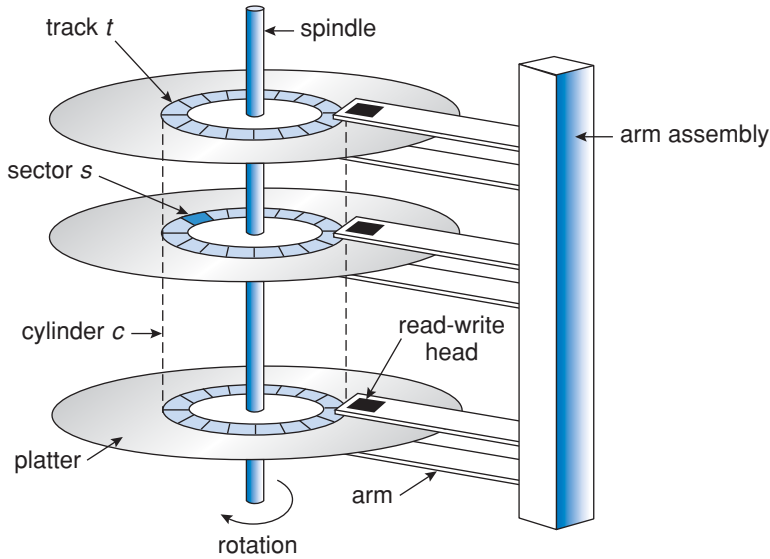
Figure 9.1 Moving-head disk mechanism.
