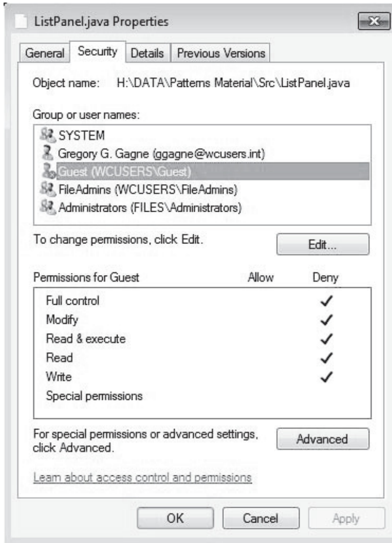
Figure 10.16 Windows 7 ® access-control list management.
