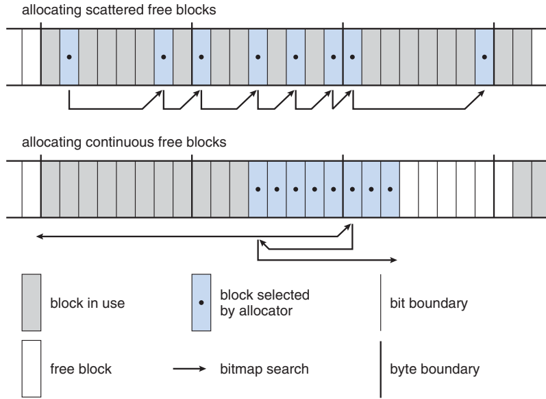
Figure 15.7 ext3 block-allocation policies.
