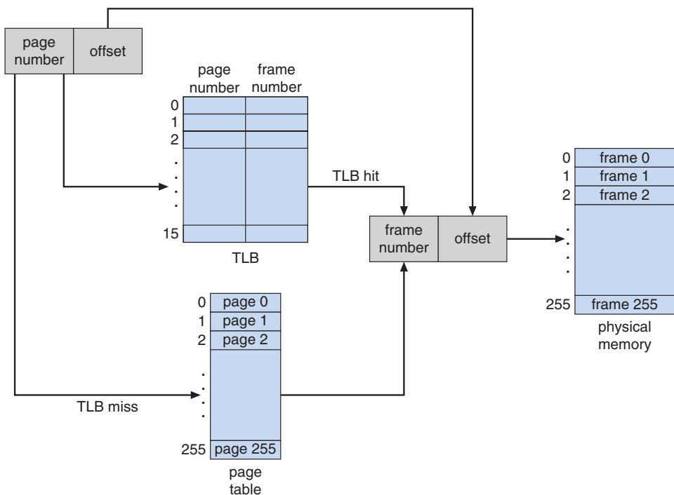
Figure 8.34 A representation of the address-translation process.
