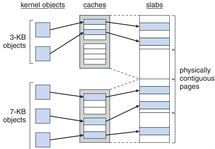
Figure 15.5 Slab allocator in Linux.
