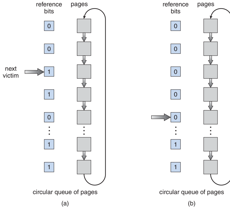
Figure 8.17 Second-chance (clock) page-replacement algorithm.
