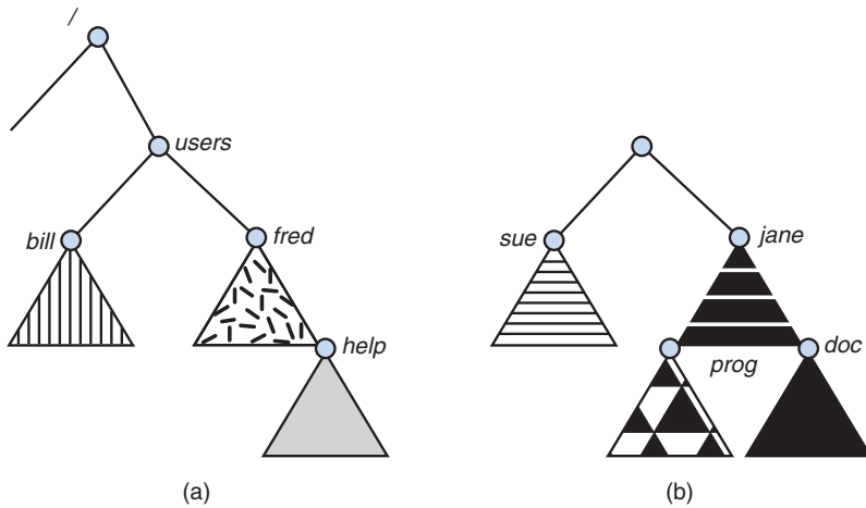
Figure 10.14 File system. (a) Existing system. (b) Unmounted volume.
