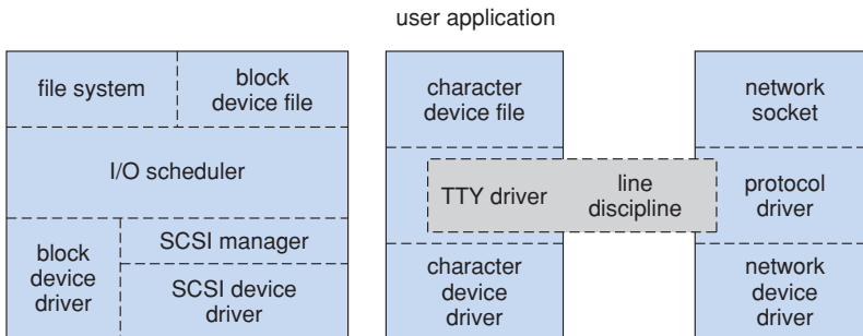
Figure 15.8 Device-driver block structure.
