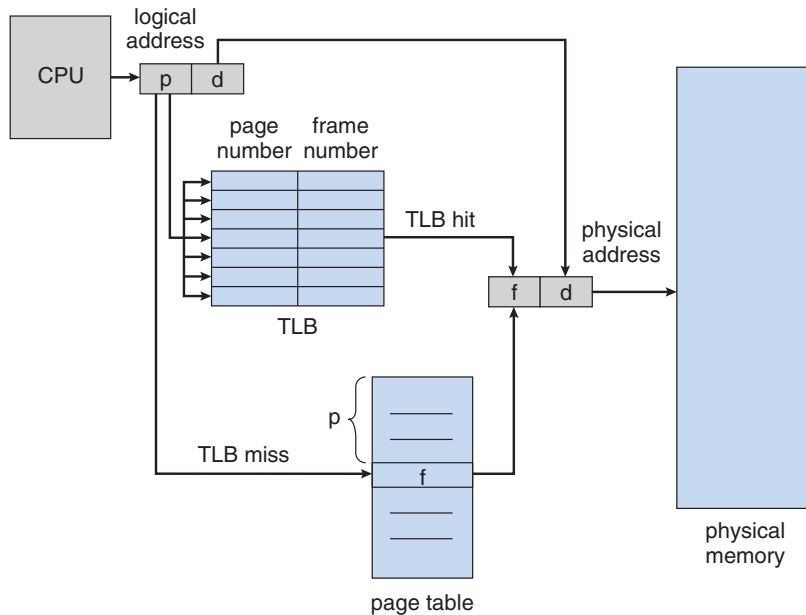
Figure 7.14 Paging hardware with TLB.
