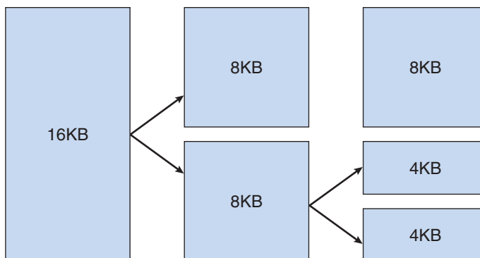
Figure 15.4 Splitting of memory in the buddy system.
