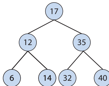
Figure 1.16 Binary search tree.
