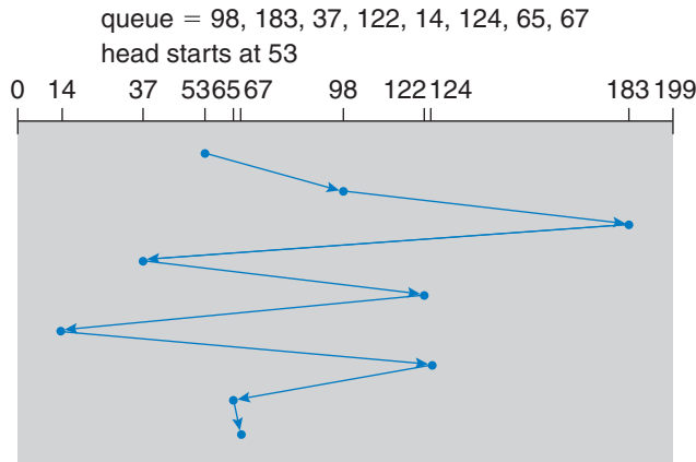
Figure 9.4 FCFS disk scheduling.
