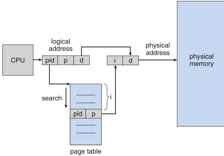
Figure 7.20 Inverted page table.
