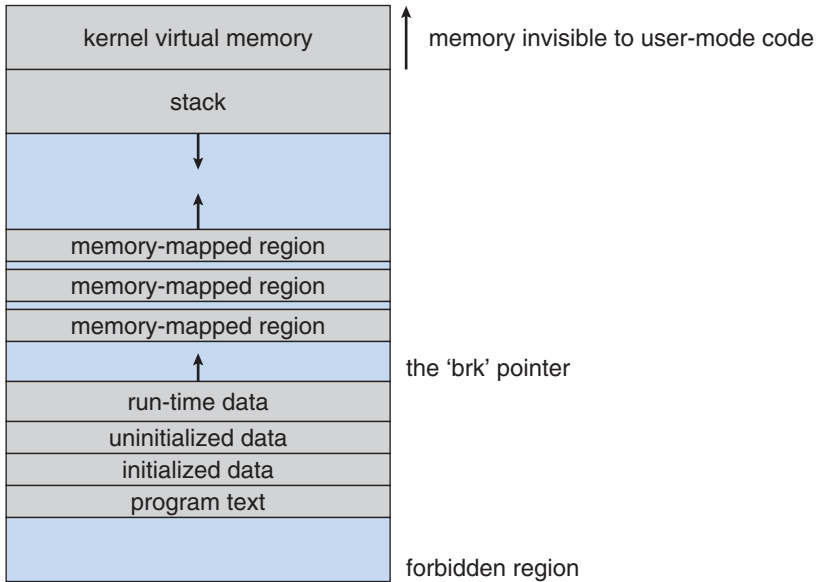
Figure 15.6 Memory layout for ELF programs.
