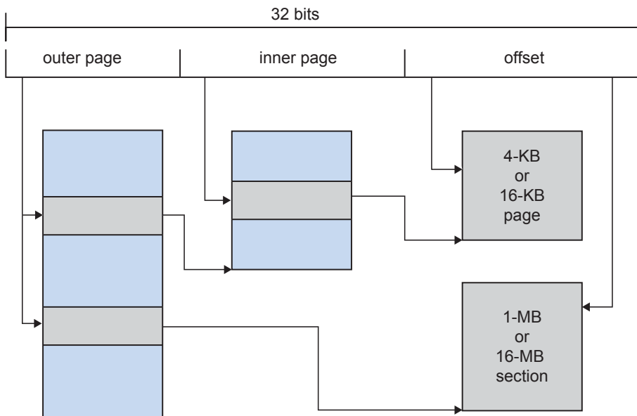
Figure 7.26 Logical address translation in ARM.
