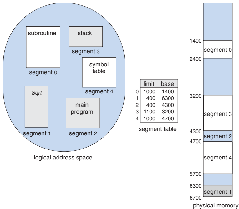
Figure 7.9 Example of segmentation.
