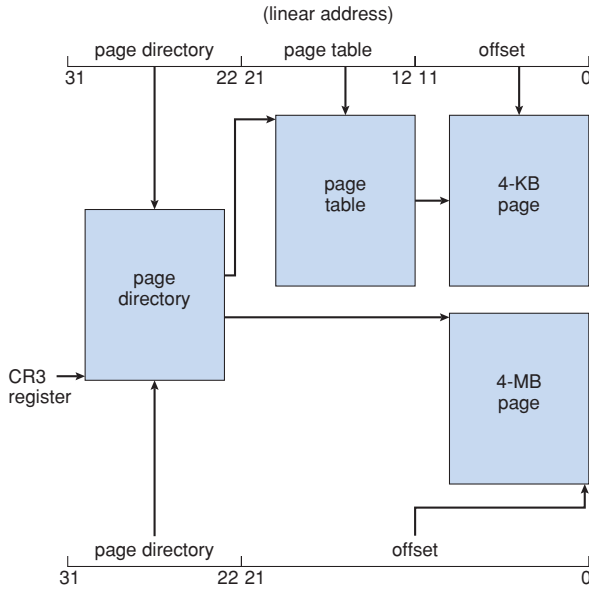
Figure 7.23 Paging in the IA-32 architecture.
