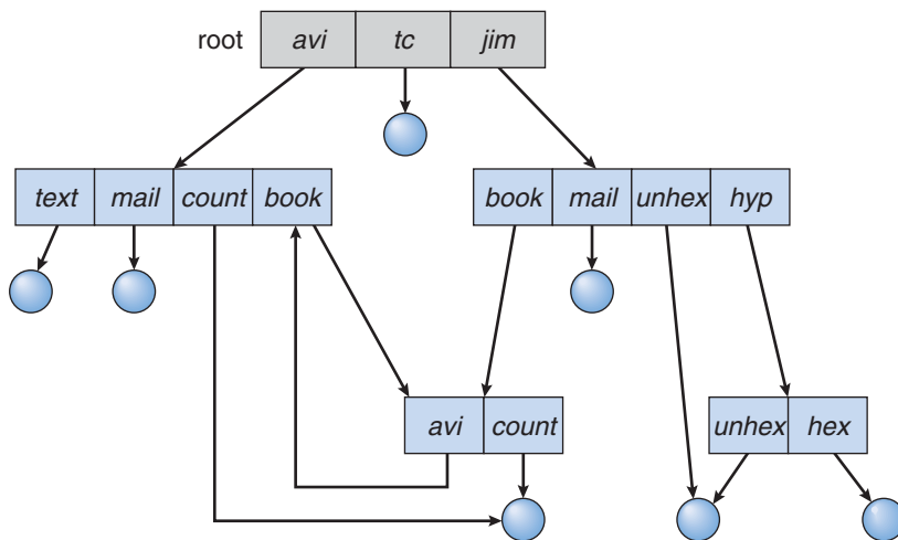
Figure 10.13 General graph directory.
