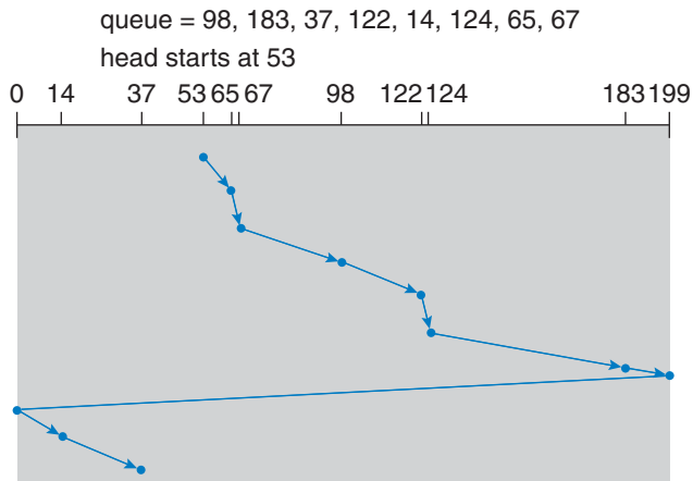
Figure 9.7 C-SCAN disk scheduling.
