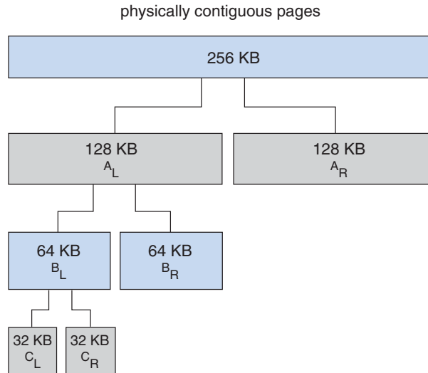
Figure 8.26 Buddy system allocation.
