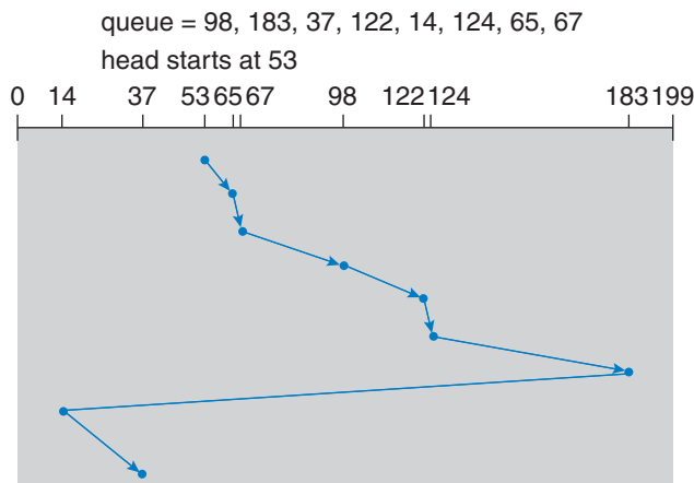
Figure 9.8 C-LOOK disk scheduling.
