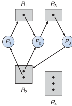
Figure 5.23 Resource-allocation graph with a deadlock.
