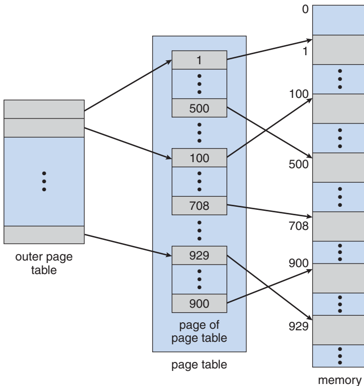
Figure 7.17 A two-level page-table scheme.
