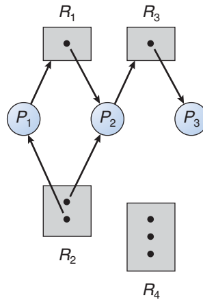
Figure 5.22 Resource-allocation graph.
