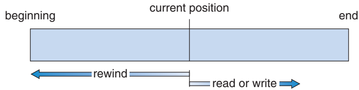
Figure 10.4 Sequential-access file.
