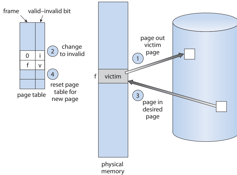
Figure 8.10 Page replacement.
