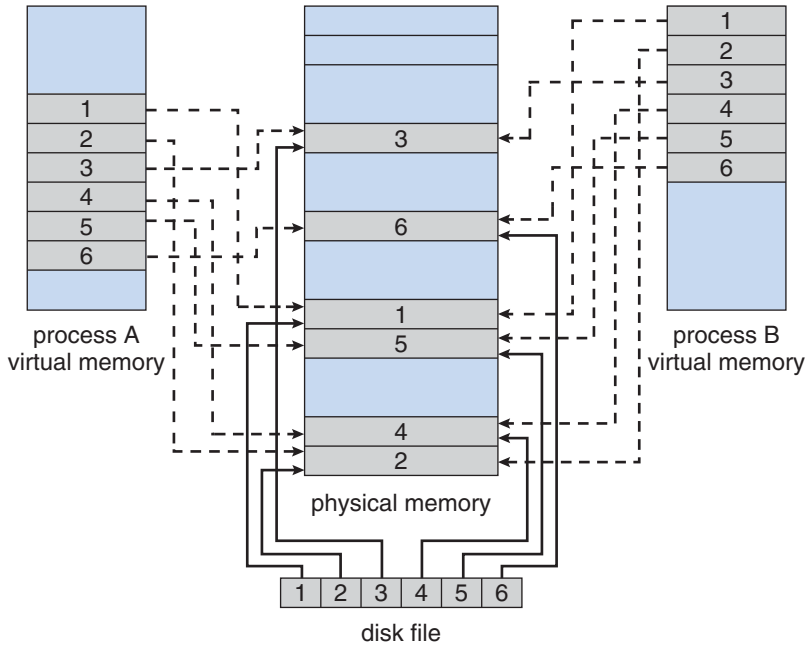
Figure 8.22 Memory-mapped files.
