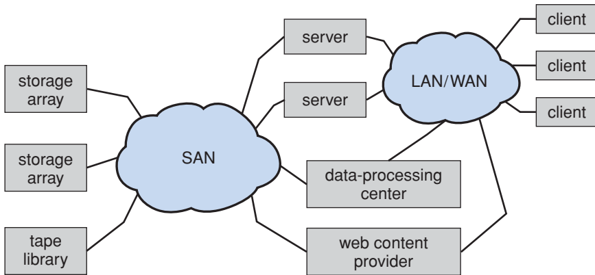
Figure 9.3 Storage-area network.
