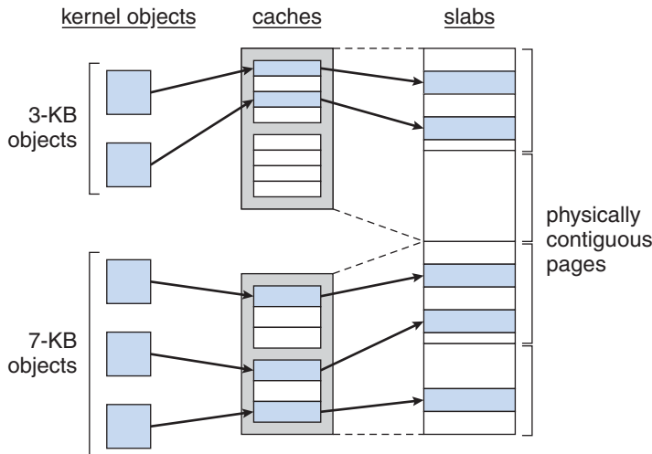
Figure 8.27 Slab allocation.
