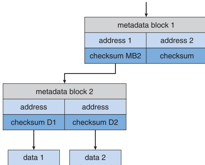
Figure 9.13 ZFS checksums all metadata and data.
