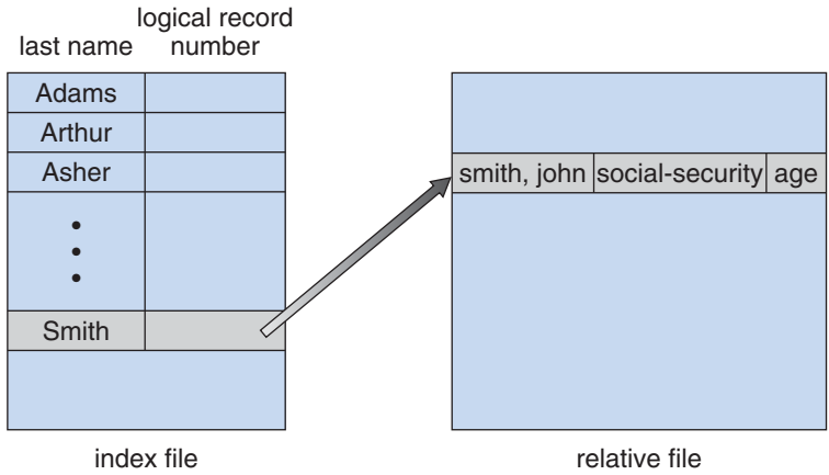
Figure 10.6 Example of index and relative files.
