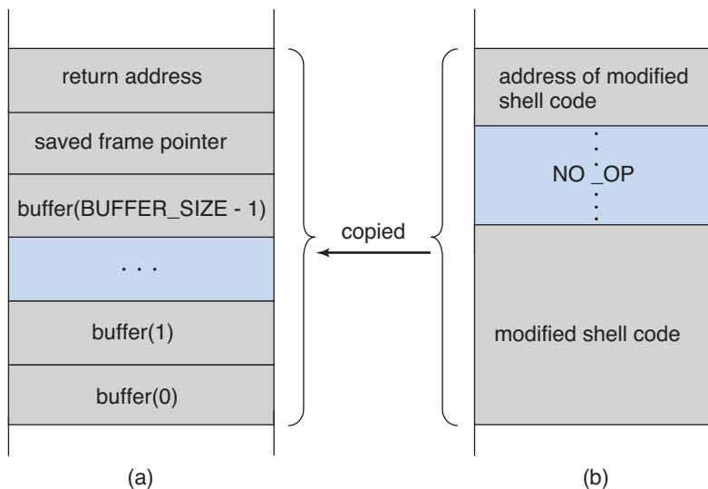
Figure 14.4 Hypothetical stack frame for Figure 14.2, (a) before and (b) after.
