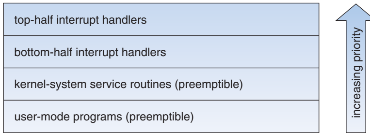
Figure 15.2 Interrupt protection levels.
