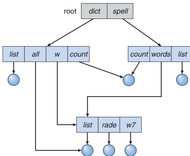
Figure 10.12 Acyclic-graph directory structure.
