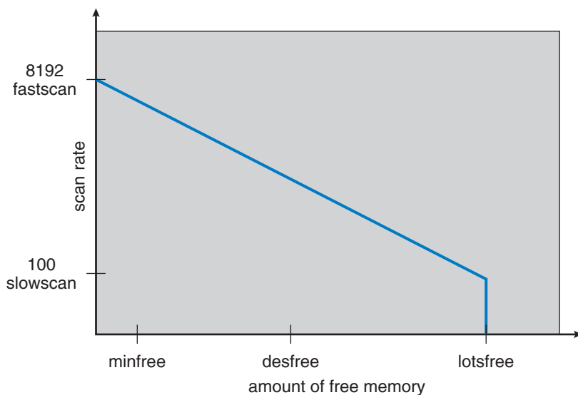
Figure 8.29 Solaris page scanner.
