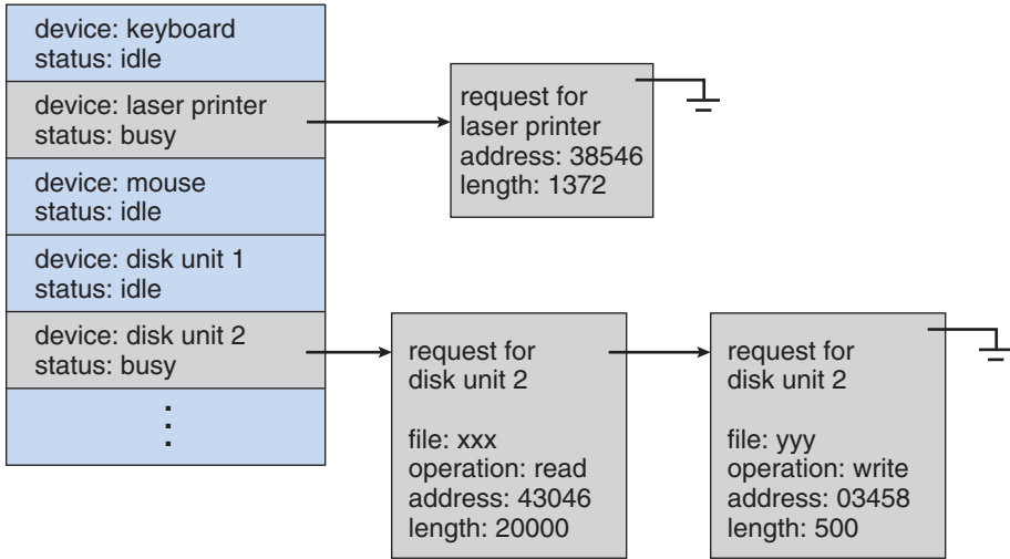
Figure 12.9 Device-status table.
