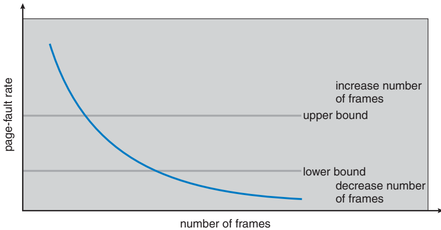
Figure 8.21 Page-fault frequency.
