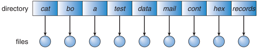
Figure 10.9 Single-level directory.
