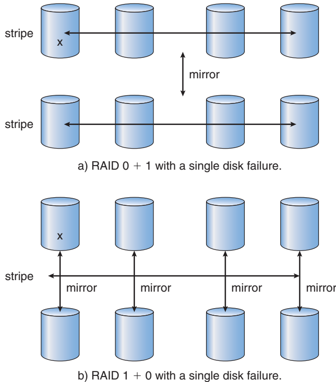
Figure 9.12 RAID 0 + 1 and 1 + 0.
