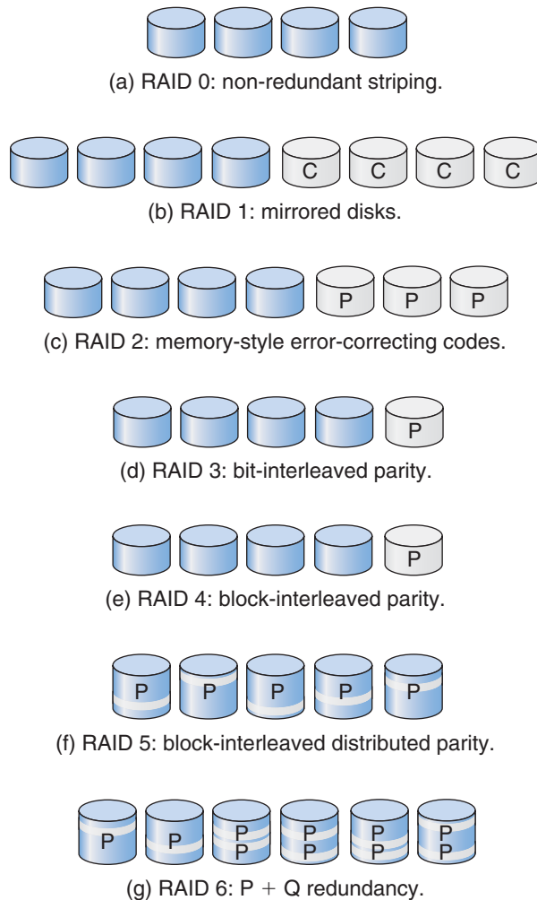
Figure 9.11 RAID levels.
