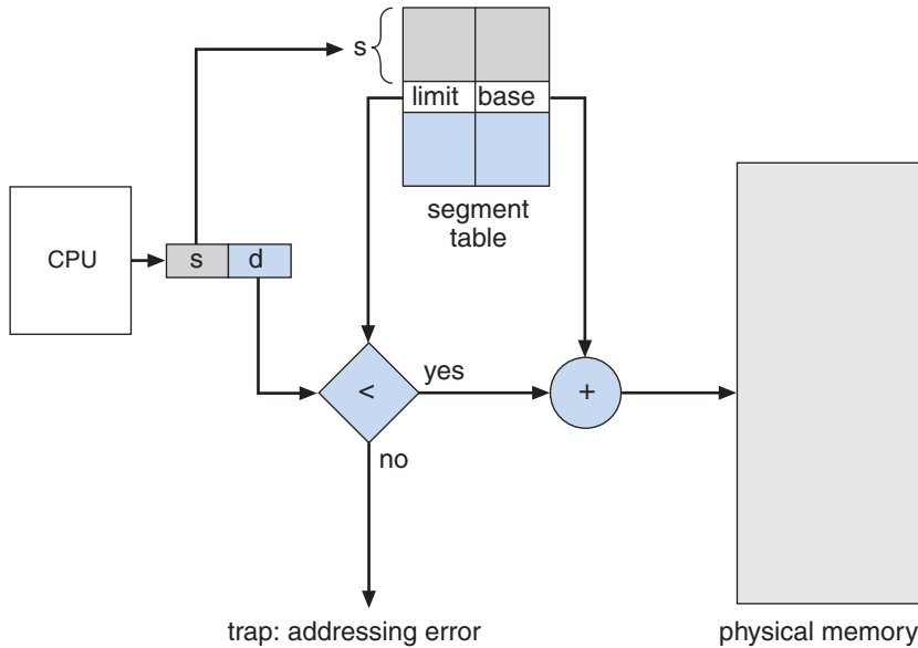
Figure 7.8 Segmentation hardware.
