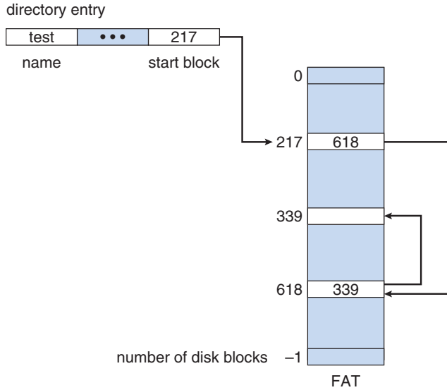
Figure 11.7 File-allocation table.
