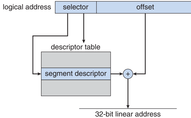
Figure 7.22 IA-32 segmentation.
