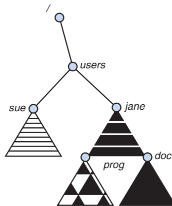
Figure 10.15 Mount point.
