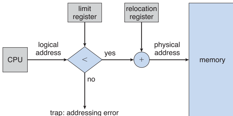
Figure 7.6 Hardware support for relocation and limit registers.
