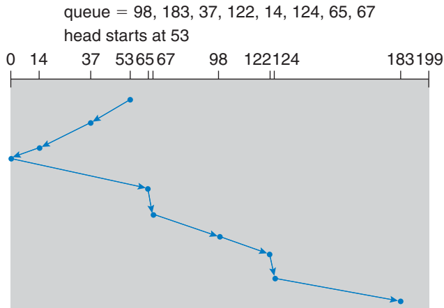
Figure 9.6 SCAN disk scheduling.
