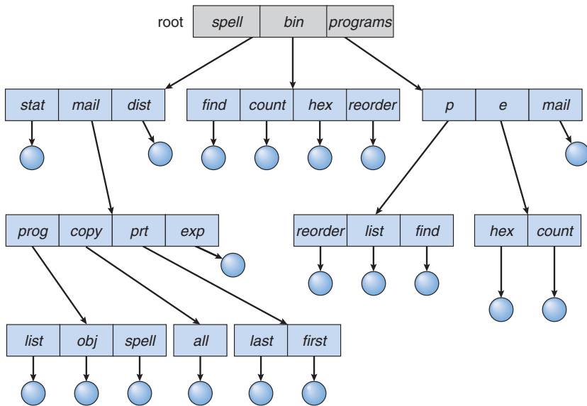
Figure 10.11 Tree-structured directory structure.
