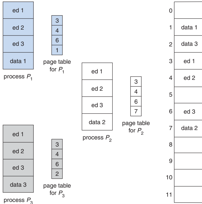
Figure 7.16 Sharing of code in a paging environment.
