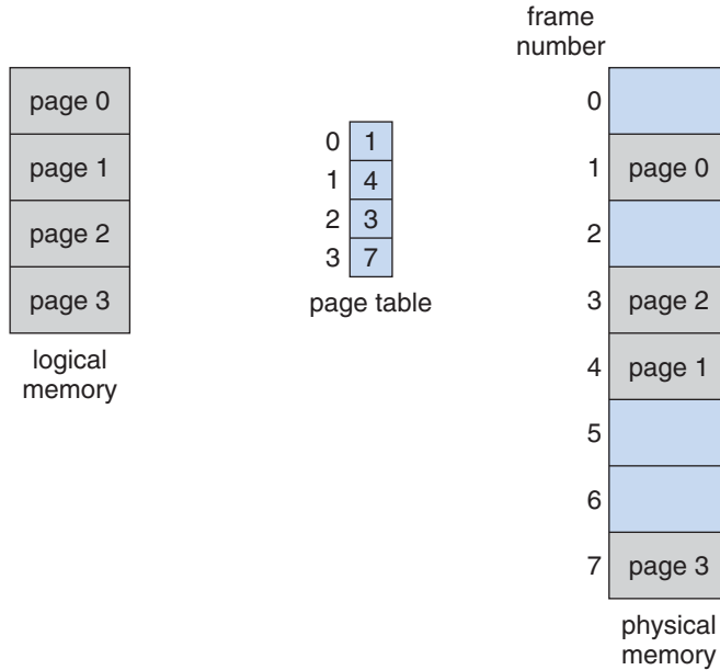
Figure 7.11 Paging model of logical and physical memory.
